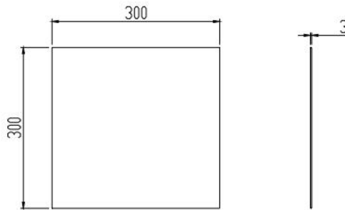
( figure 4 ) Aluminum Radiator Size
